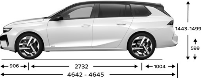
Astra Sports Tourer Alle Masse in mm
